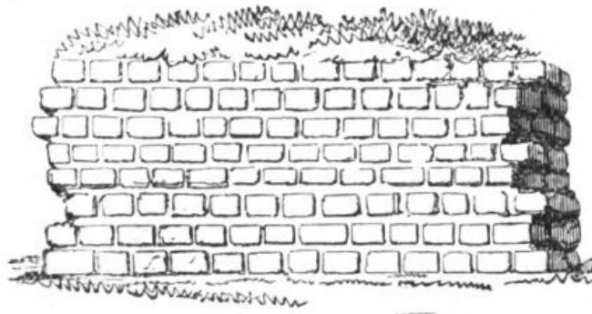
LONGITUDINAL SECTION OF THE ROMAN WALL.
