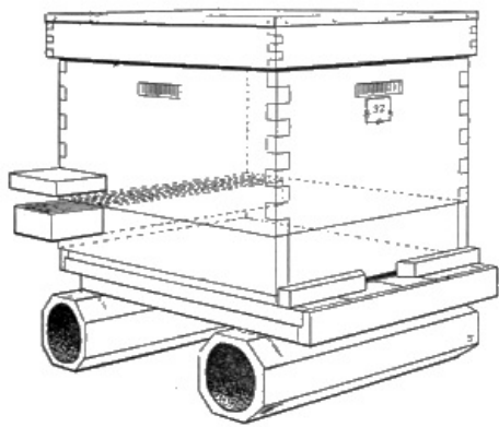
FIG. 18.—Feeder set in collar under hive body.
