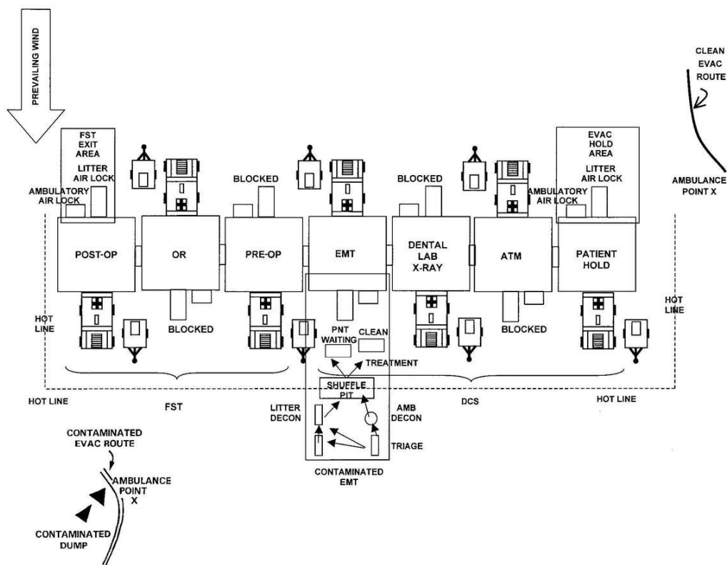
Figure F-4. Forward surgical team and division clearing station configuration for operations in a nuclear, biological, chemical environment.
