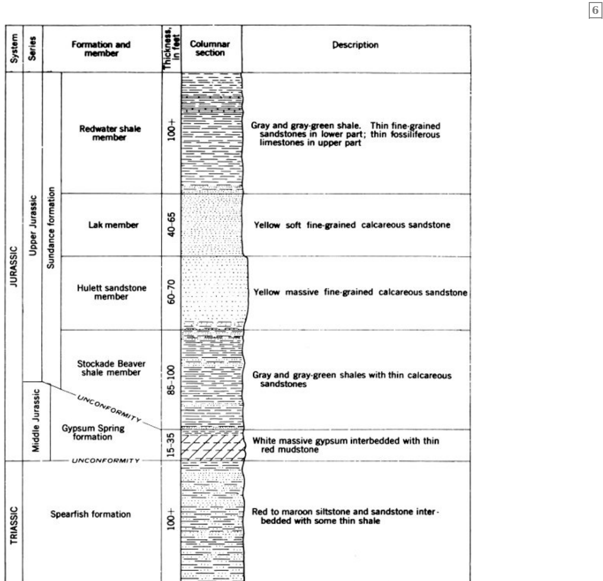
FIGURE 54.—Generalized section of the sedimentary rocks of the Devils Tower National Monument.
