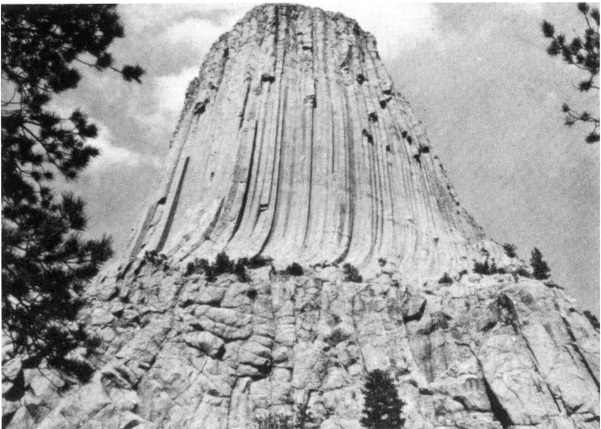
FIGURE 53.—B. Southwest corner of Devils Tower showing the columns flaring out and merging to form the massive base.
