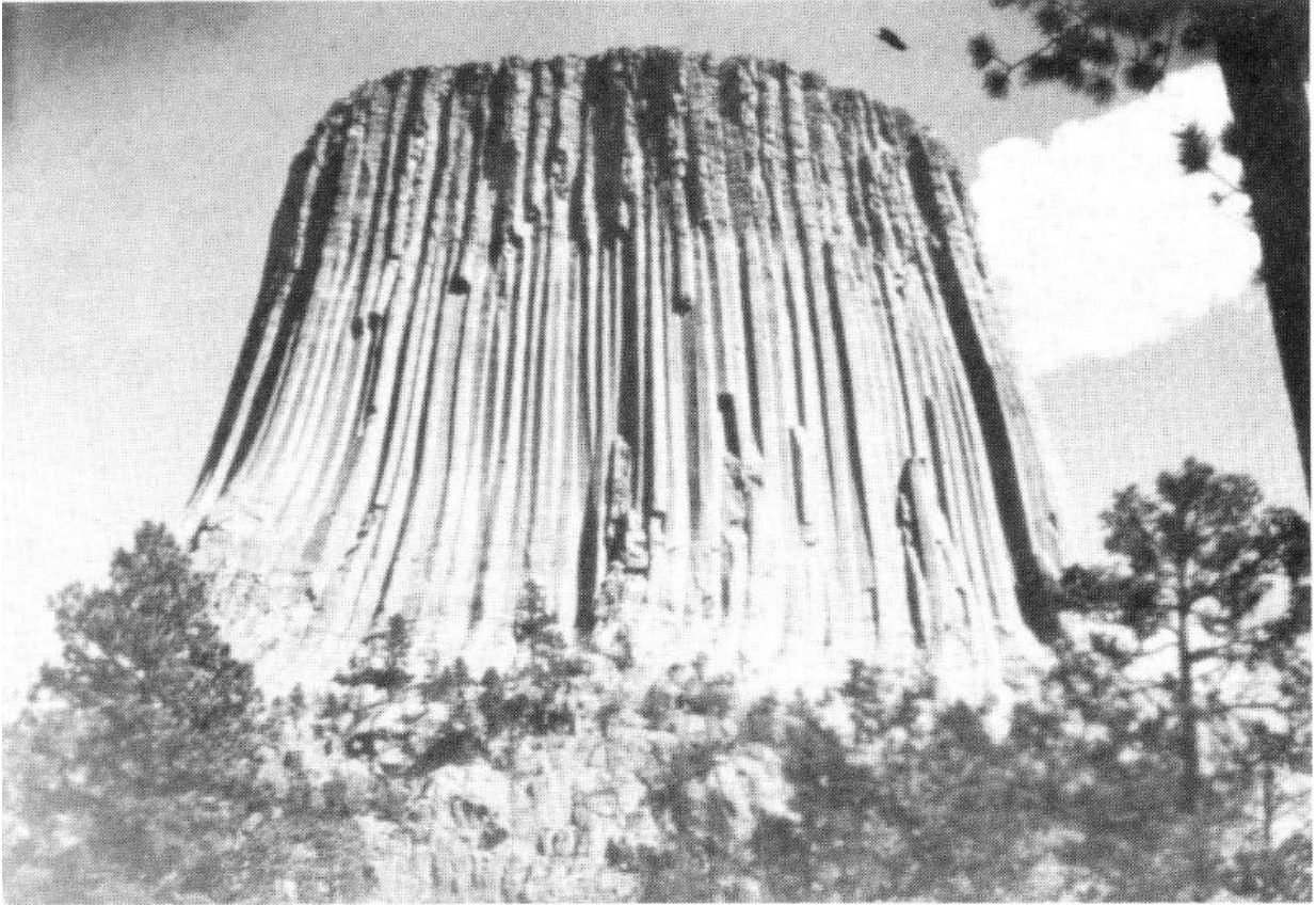
FIGURE 53.—A. Northwest side of Devils Tower showing how the columns taper or converge and in places unite near the top and are cut by numerous cross-fractures.
