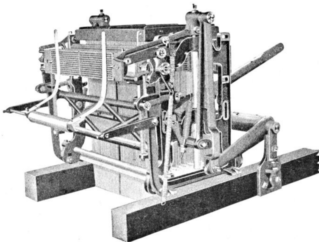
Fig. 9. Single Action Jacquard Machine.
