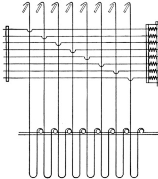
Fig. 4. Common Jacquard Hook.
