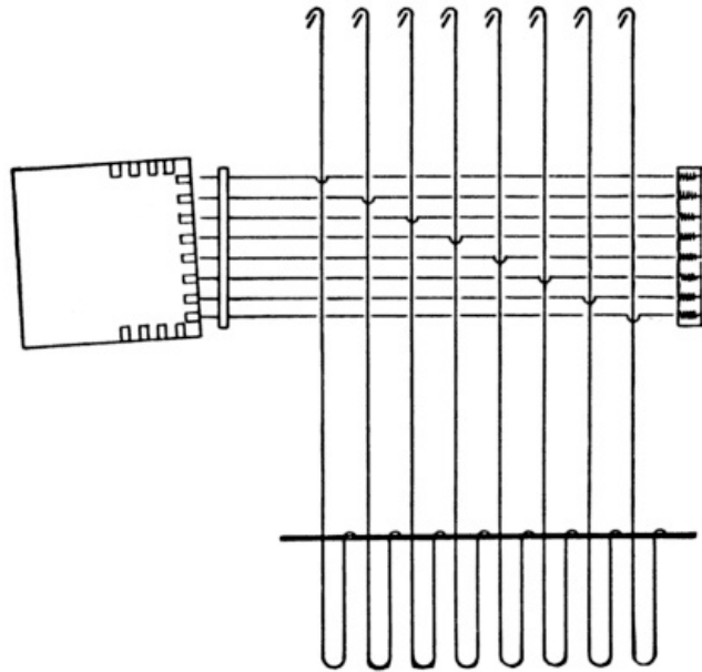
Fig. 18. Cylinder Out of True with Needle Board.
