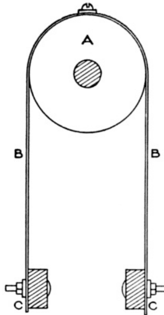
Fig. 30. Pulley and Belt for Lifting Griffe.
