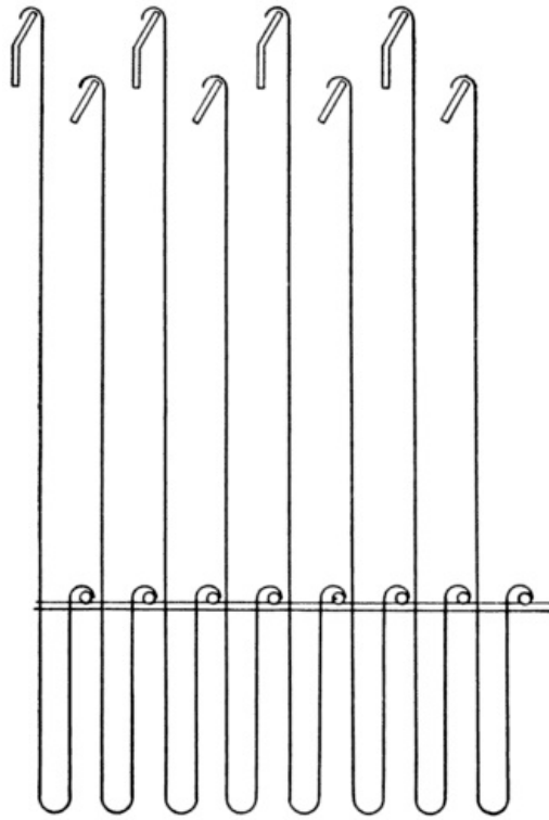
Fig. 6. Alternate Arrangement of Griffe Blades.
