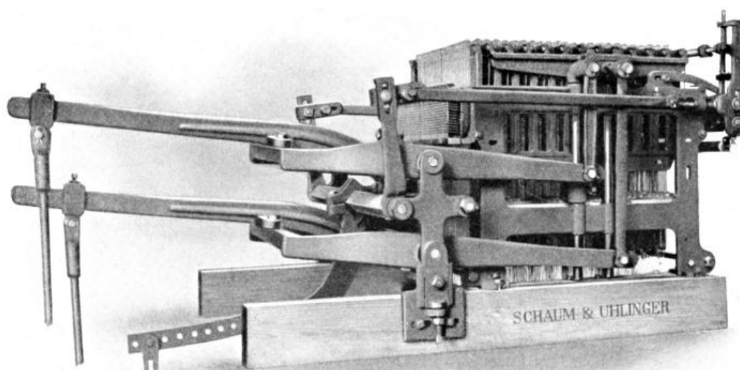
Fig. 22. Double-Lift and Single Cylinder Machine.
