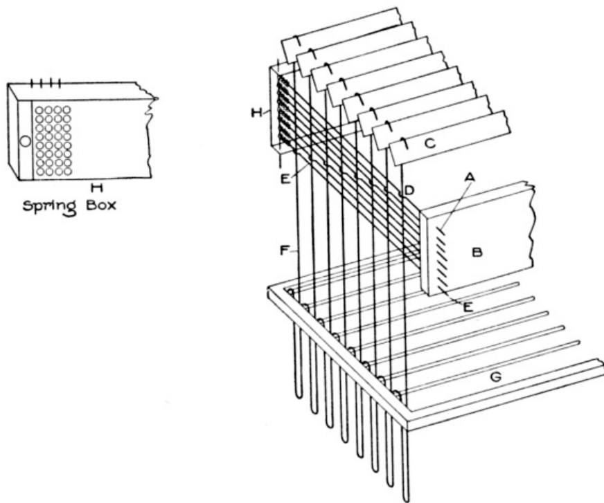
Fig. 10. Showing Arrangement of Hooks, Needles, Etc.
