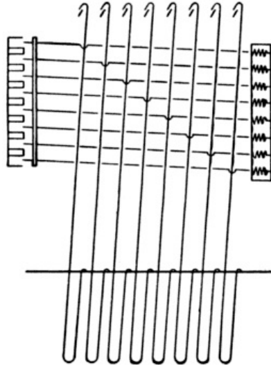
Fig. 12. Hooks Out of Perpendicular with Needles.
