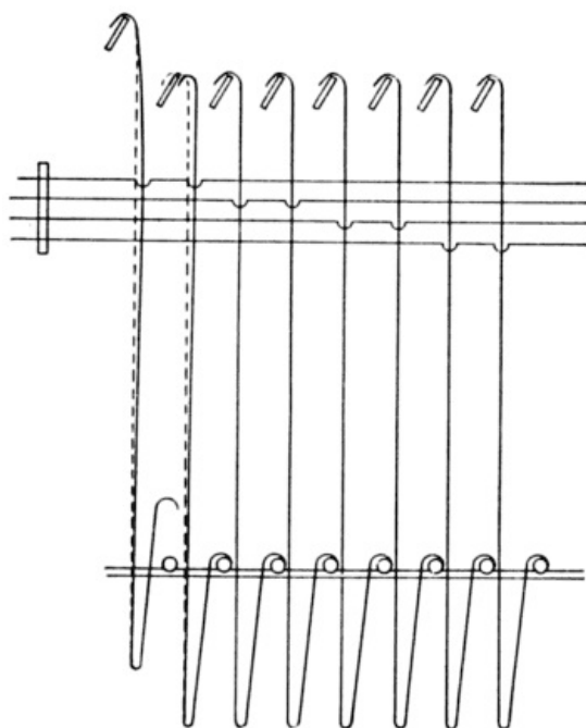
Fig. 23. Needles and Hooks Used in Double-Lift
