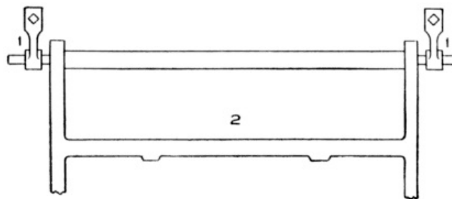
Fig. 19. Iron Bar Supporting Batten Frame.
