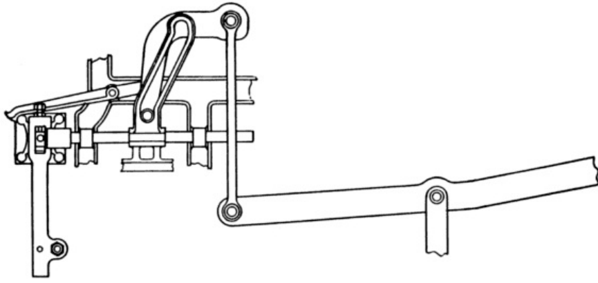
Fig. 20. Spindle Cylinder Motion.
