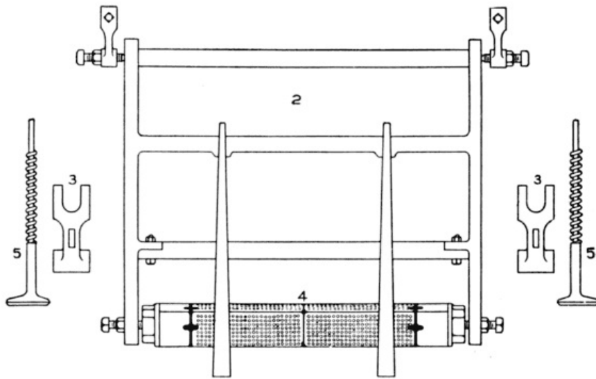
Fig. 16. Details of Batten or Swing Cylinder Motion.
