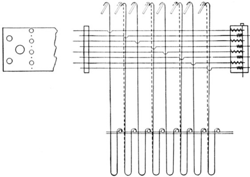
Fig. 8. Hooks Used at the Present Time.
