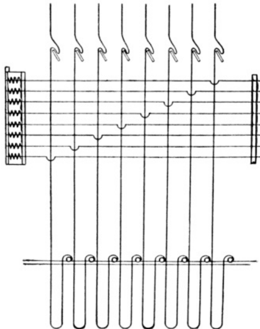
Fig. 7. Showing Hook Extending Above Griffe.
