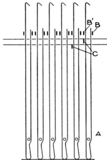
Fig. 3. Hook Sometimes Used on French Machines.
