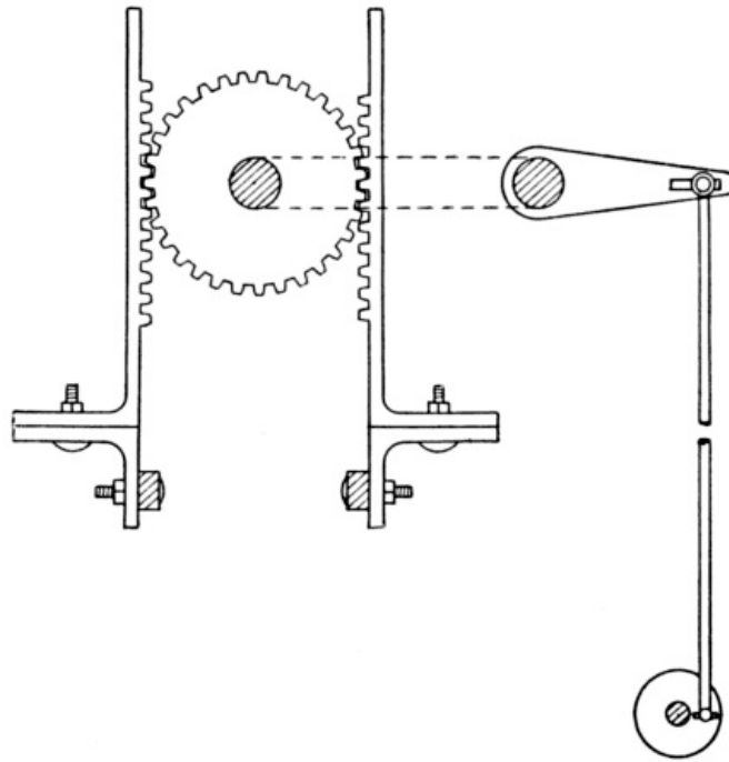
Fig. 29. Rack Method of Lifting Griffe.
