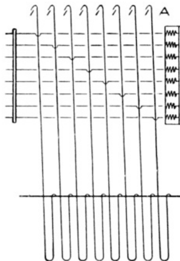
Fig. 13. Hooks Out of Perpendicular with Needles.
