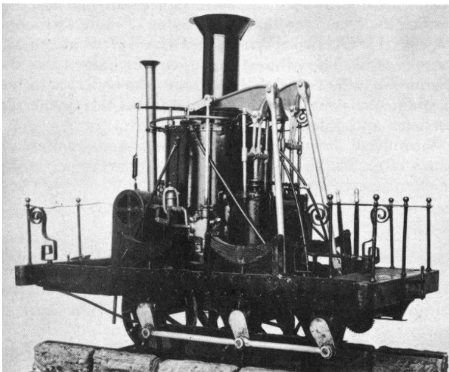
Figure 65.—Model of Davis and Gartner Arabian , 1834.
