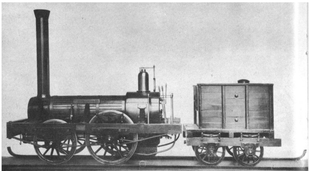
Figure 64.—Model of Baldwin Old Ironsides , 1832.
