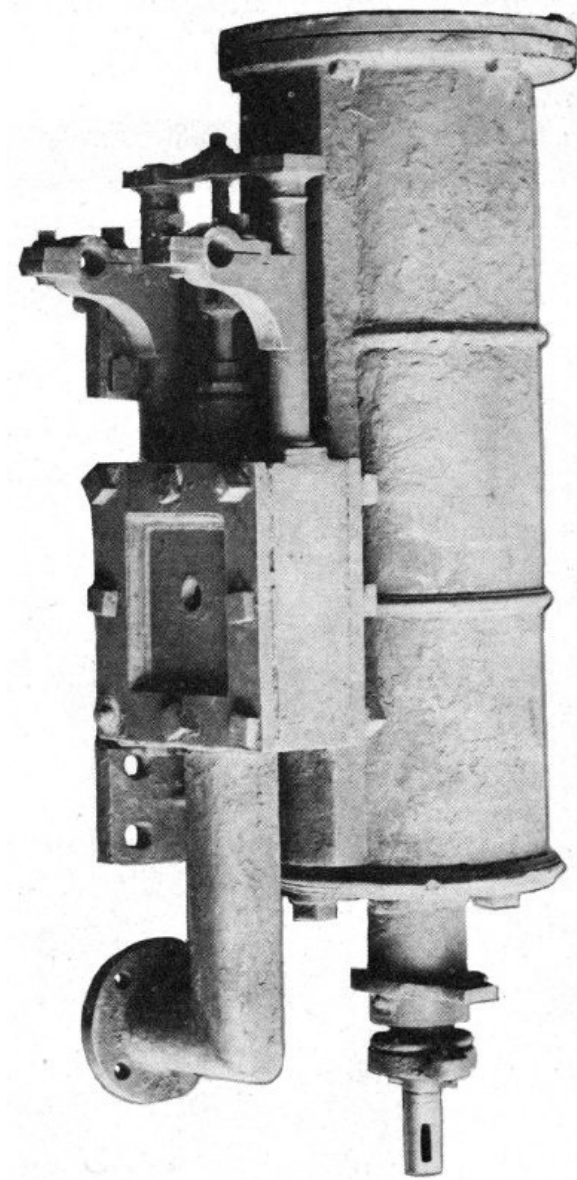
Figure 8.—Cylinder of America , in National Museum.
