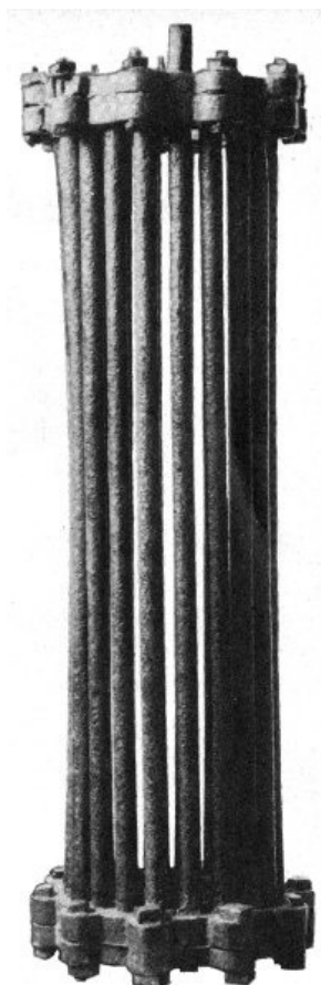
Figure 1.—Original boiler, now in National Museum, of experimental locomotive built in 1825 by Col. John Stevens.
