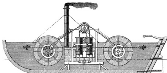
SYMINGTON'S FIRST STEAMBOAT ENGINE.
