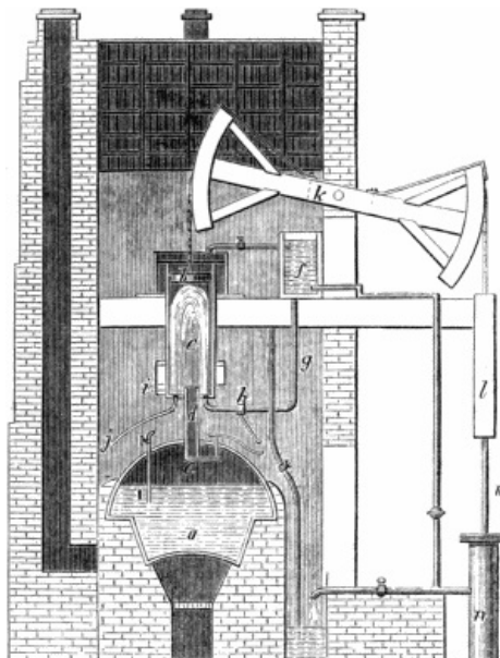
NEWCOMEN'S ENGINE. [44]
