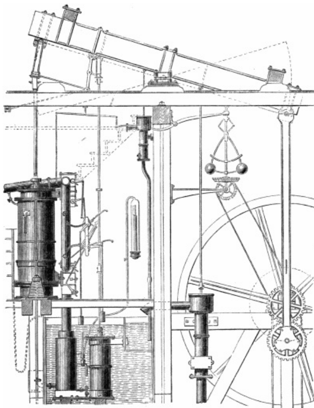
DOUBLE-ACTING ENGINE, ALBION MILL.
