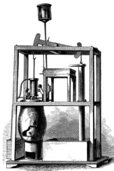
THE NEWCOMEN MODEL.
