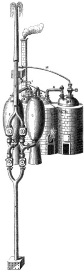
SAVERY'S ENGINE.
