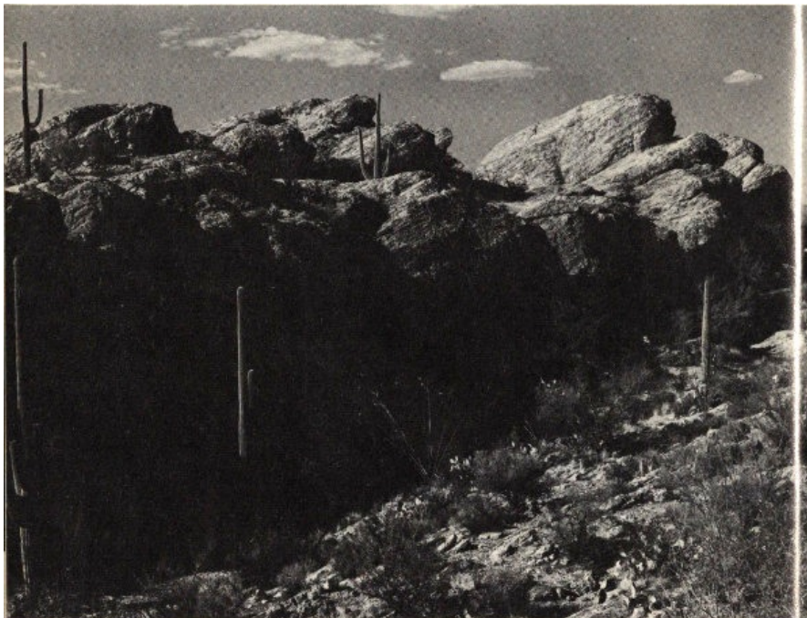
Banded augen gneiss on Cactus Forest Drive. Javelinas formerly took refuge from the sun in the dens under these overhanging rocks.
