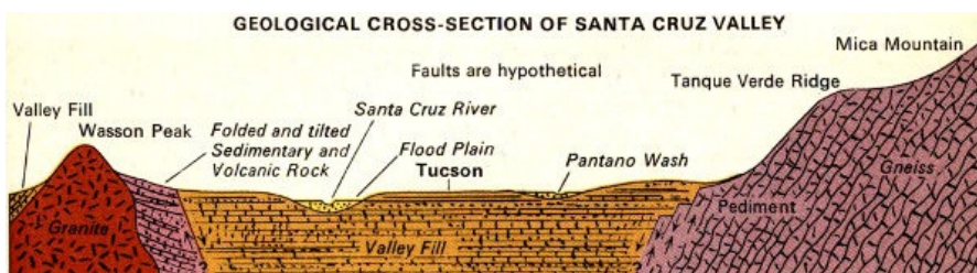
GEOLOGICAL CROSS-SECTION OF SANTA CRUZ VALLEY
