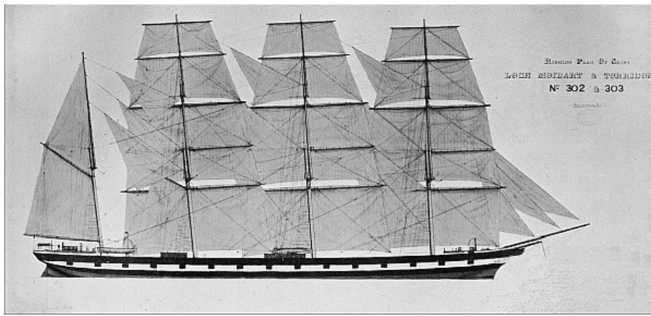
SAIL PLAN OF "LOCH MOIDART" AND "LOCH TORRIDON."
