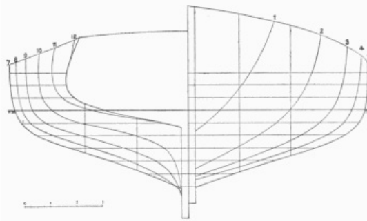
Body-plan of the Spray.
