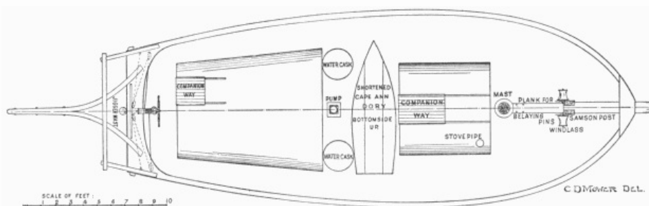
Deck-plan of the Spray .
