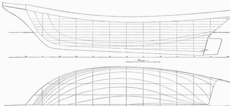
Lines of the Spray.
