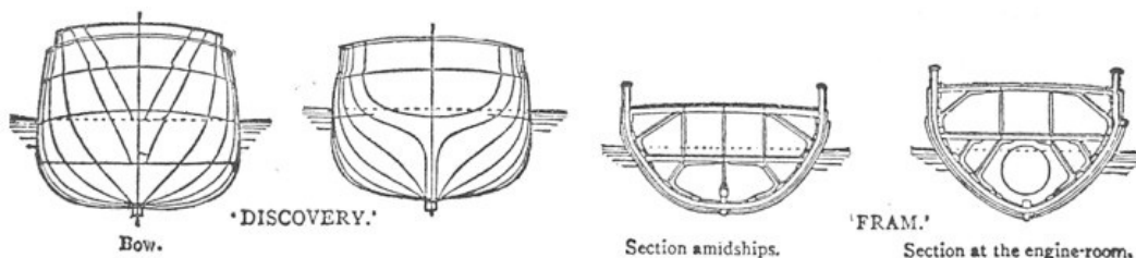
OUTLINE DRAWINGS OF 'DISCOVERY' AND 'FRAM'.
