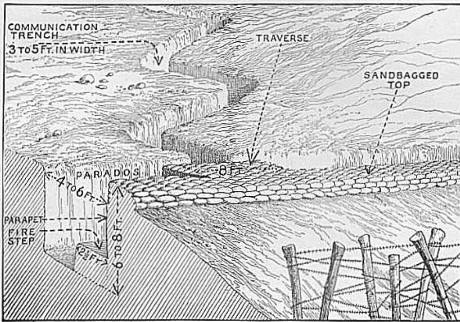
Diagram Showing Typical Front-Line and Communication Trenches.
