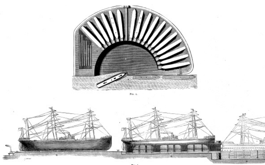
Fig. 1. IMPROVED FLOATING PONTOON DRY DOCK.
