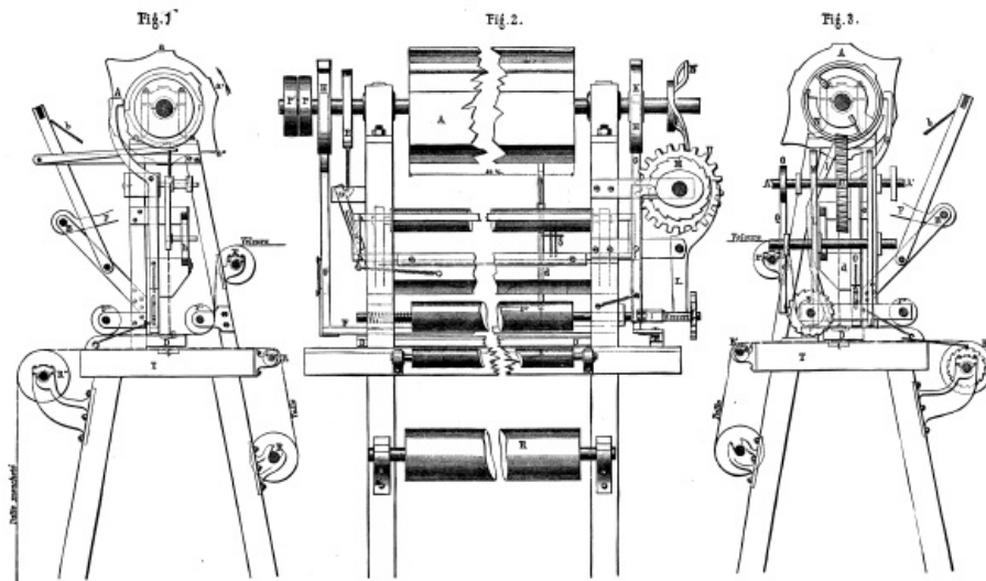
IMPROVED MACHINE FOR DOTTING TULLAND OTHER LIGHT FABRICS.
