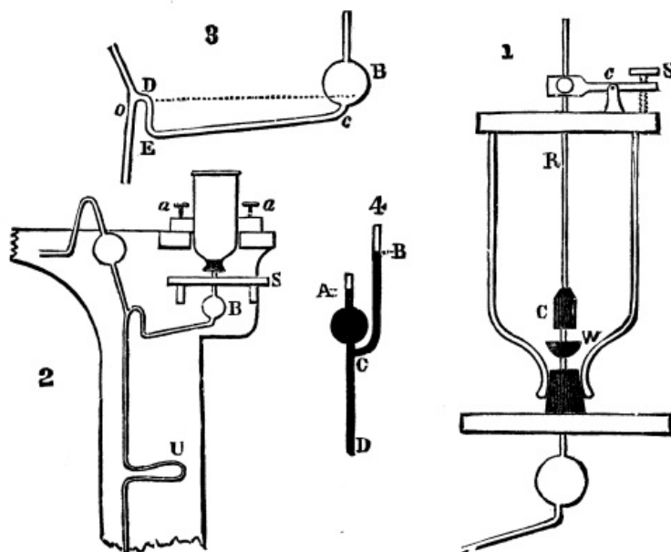
MODIFIED FORM OF SPRENGEL PUMP.
