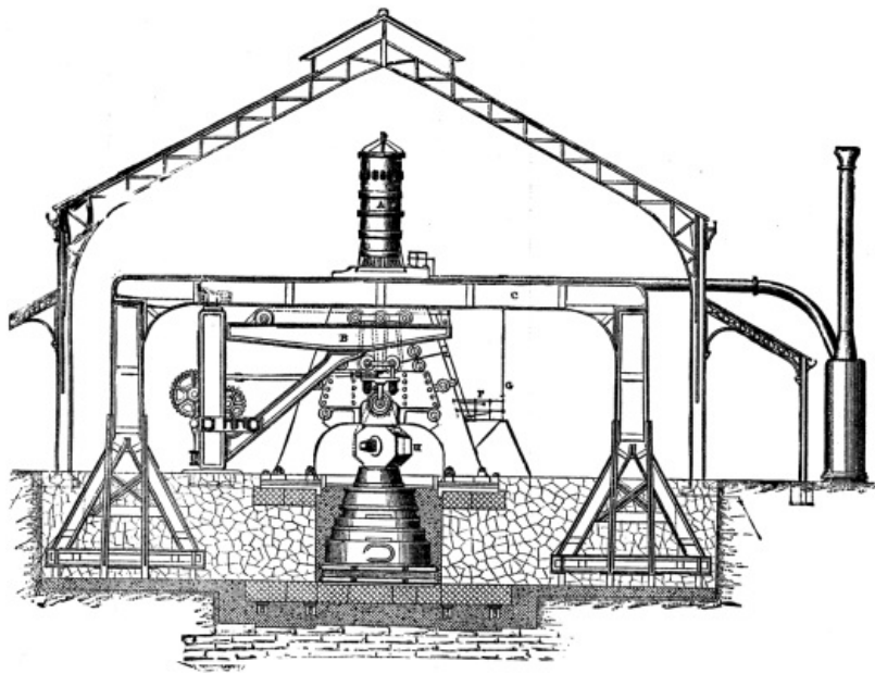
FIG. 1.--TRANSVERSE SECTION.
