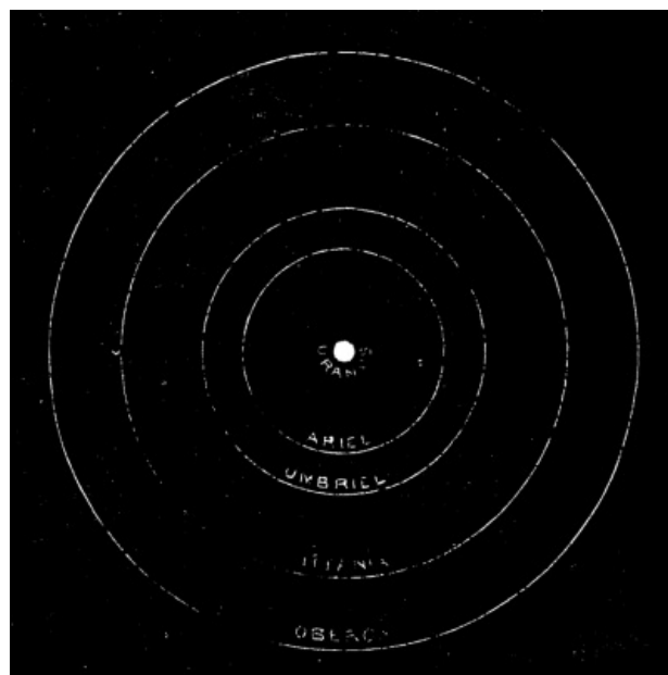
Fig. 2.--ORBITS OF THE URANIAN SATELLITES.
