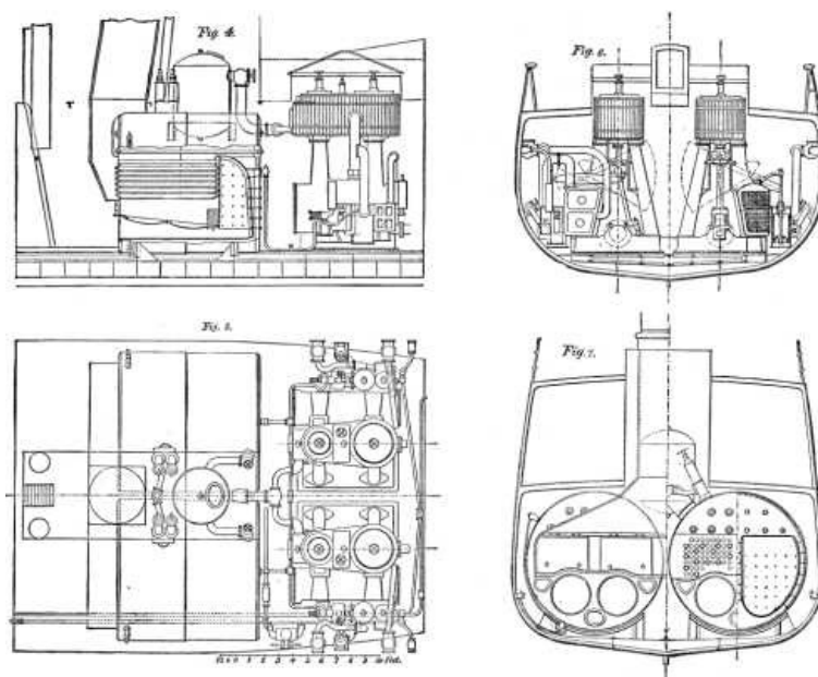
ENGINES AND BOILERS OF THE NEW STEAMSHIP CHURCHILL.
