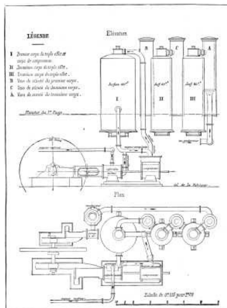
THE WEIBEL-PICCARD EVAPORATION APPARATUS.
