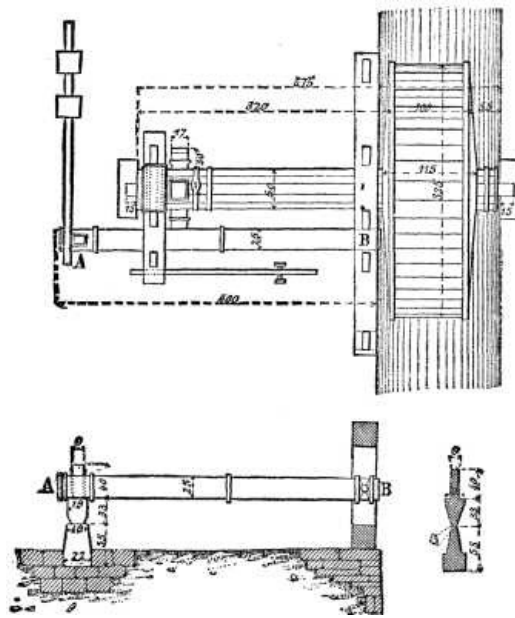
FIG. 4.--THE TRIP HAMMER.
