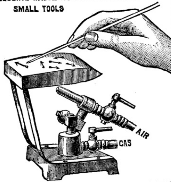
FIG. 3. BLUEING WATCH HANDS & TEMPERING SMALL TOOLS
