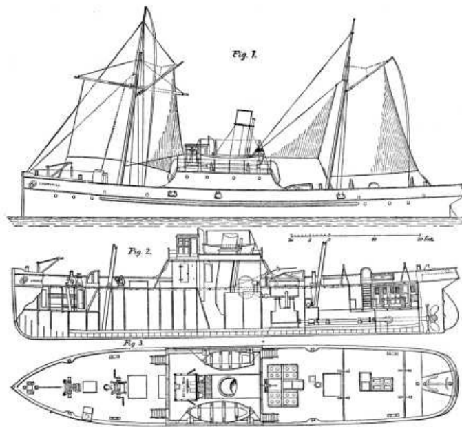
THE NEW STEAMSHIP CHURCHILL.
