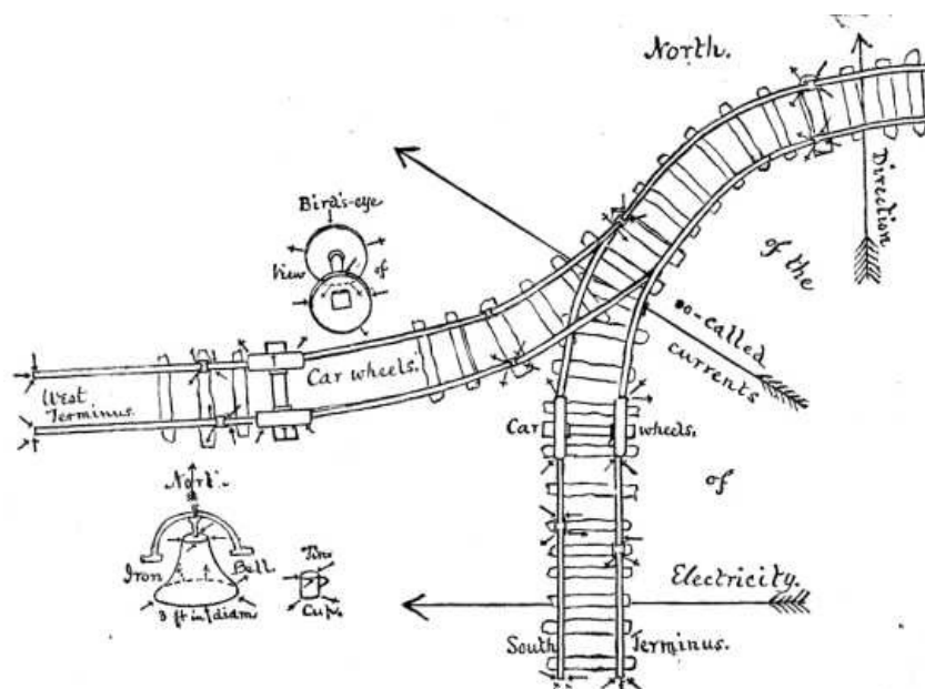
MAGNETISM ON RAILWAYS.
