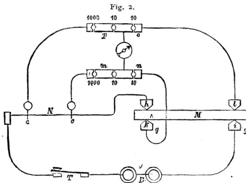
FIG. 2.--DIAGRAM SHOWING ELECTRICAL CONNECTIONS OF BRIDGE.
