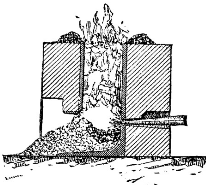
FIG. 6.--CADINHE IN OPERATION.
