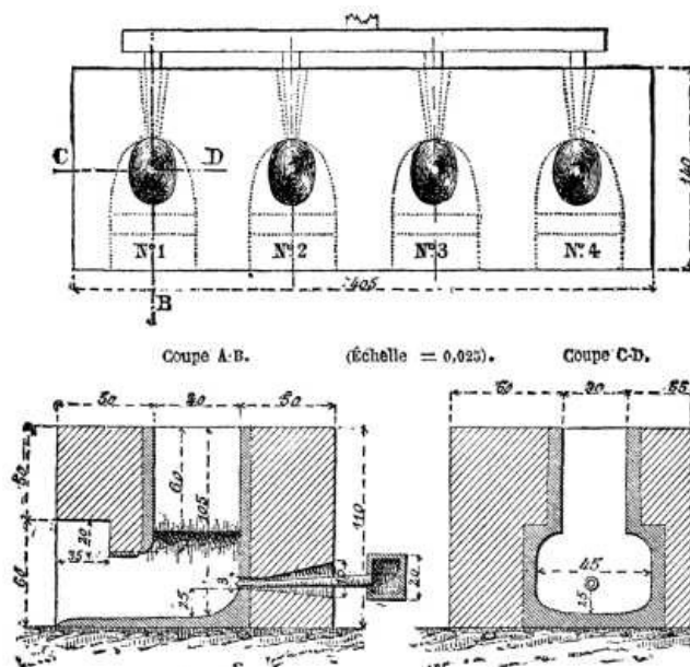
FIG 2.--FOUR-CRUCIBLE FURNACE; (PLAN).
