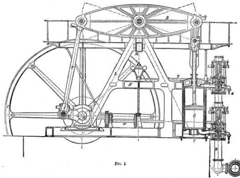
BORSIG'S IMPROVED COPOUND BEAM ENGINE. FIG. 1
