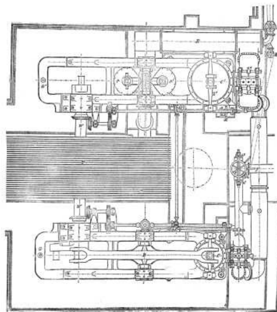
BORSIG'S IMPROVED COPOUND BEAM ENGINE. FIG. 3
