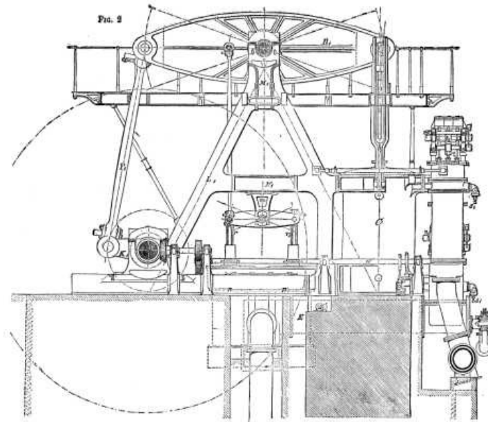
BORSIG'S IMPROVED COPOUND BEAM ENGINE. FIG. 2
