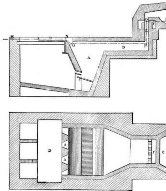
THE BICHEROUX SYSTEM OF FURNACE.
