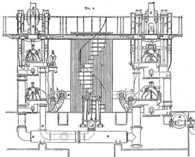
BORSIG'S IMPROVED COPOUND BEAM ENGINE. FIG. 4
