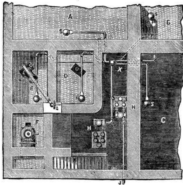
Fig. 1.--LAW AND CHATTERTON'S WATER-SOFTENING APPARATUS.
