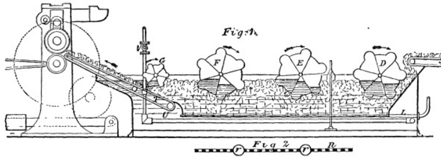
IMPROVED WOOL WASHING MACHINE.
