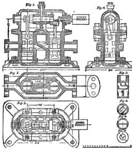
SCHMID'S WATER METER.
