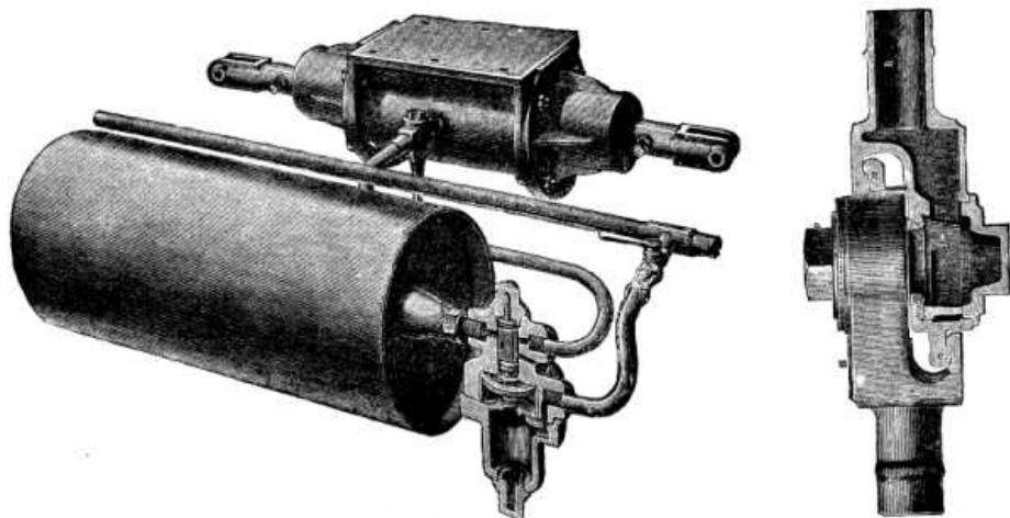
THE WESTINGHOUSE BRAKE.
