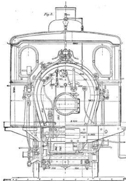
ST. GOTHARD LOCOMOTIVES.
