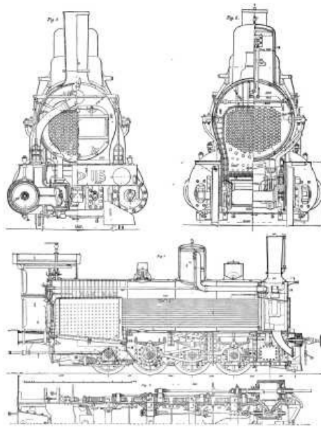
LOCOMOTIVES FOR ST. GOTHARD RAILWAY.
