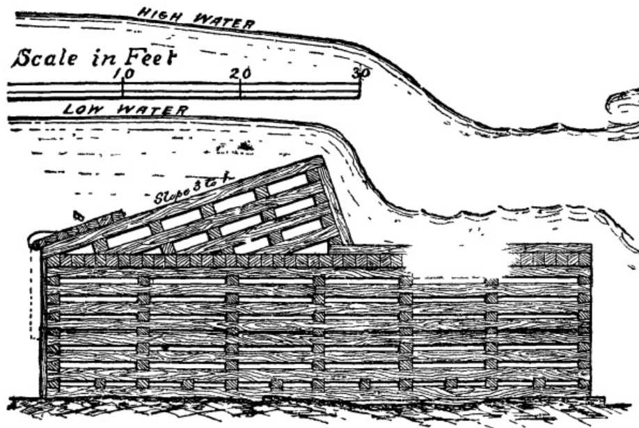
Fig. 1. CROSS SECTION IN DEEP WATER.
