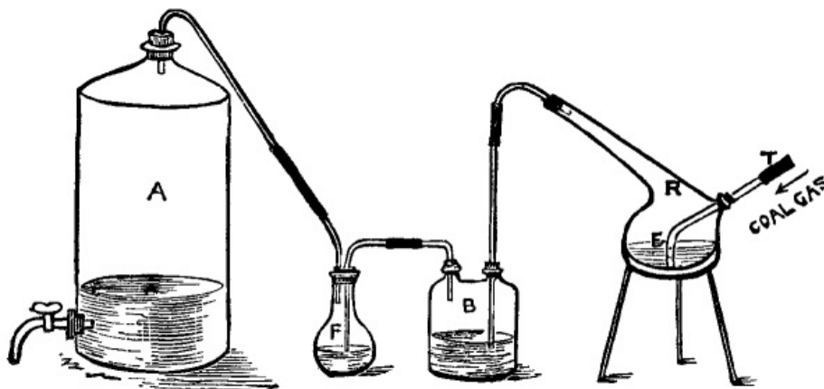
PREPARATION OF HYDROGEN SULPHIDE FROM COAL-GAS.
