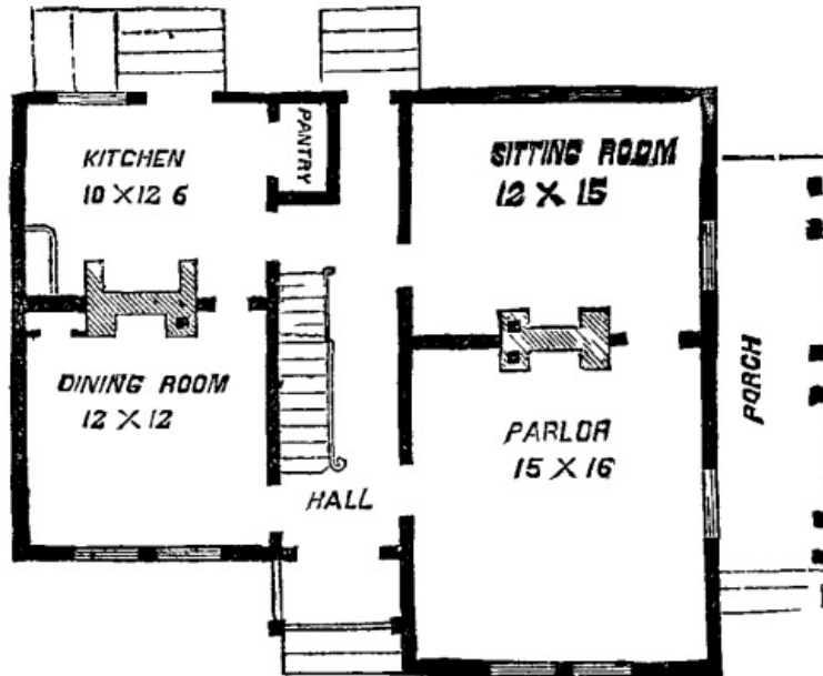
A MANSARD ROOF DWELLING. First Floor.
