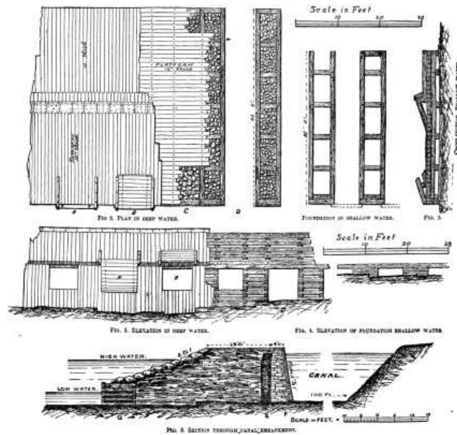
DETAILS OF THE OTTAWA RIVER DAM, AT CARILLON.
