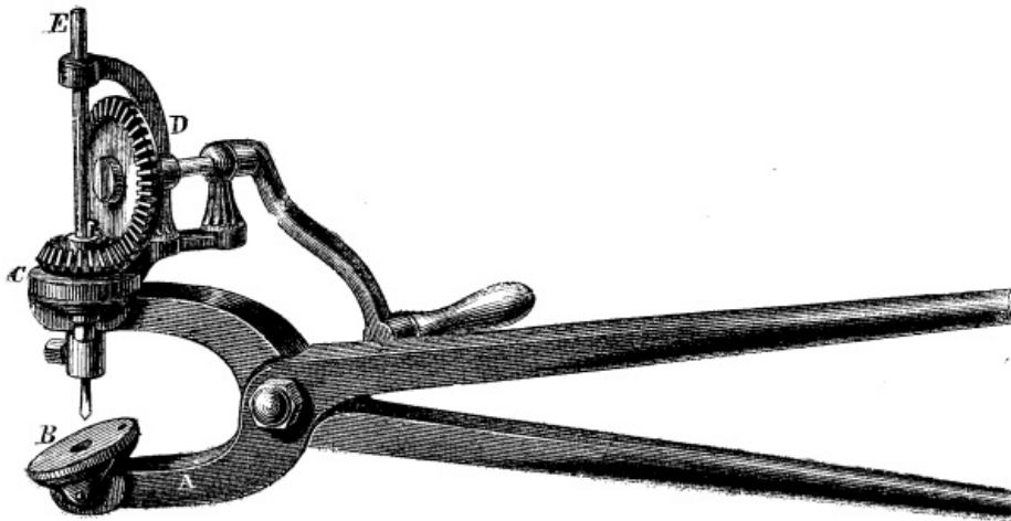
NEVERGOLD & STACKHOUSE'S TONGS DRILL.
