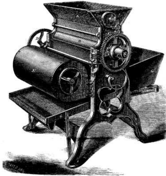
DONALDSON'S PATENT HOMINY MILL.
